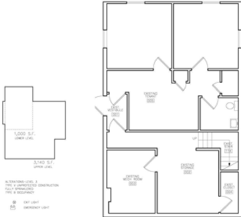
LOWER LEVEL PLAN SCALE: 1/8"=1'-0"
